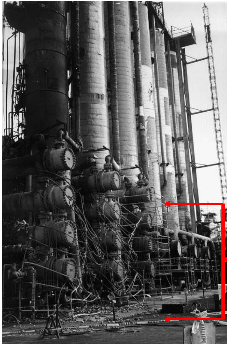
Figure 1 – Reactors with Damaged Scaffolding
